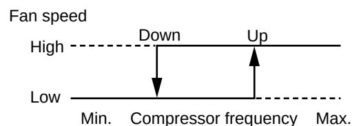
<Relation between compressor frequency and fan speed>
